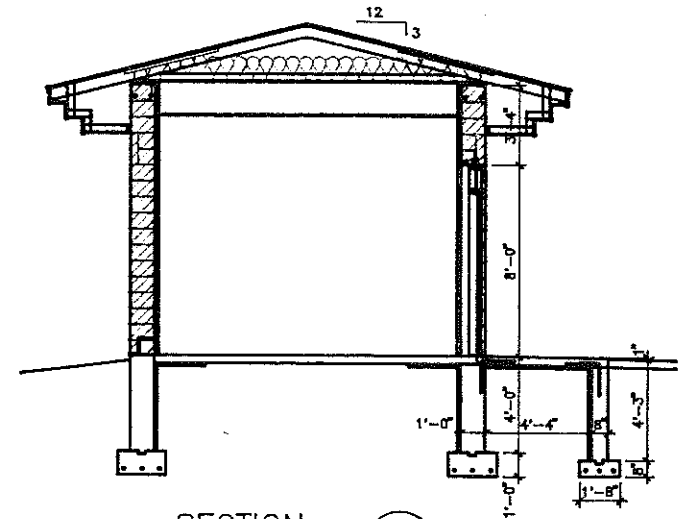
SECTION 3 1/4" = 1'-0" A202
