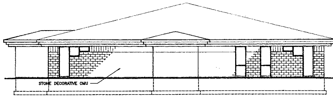
EAST ELEVATION 1/8" = 1'-0"
