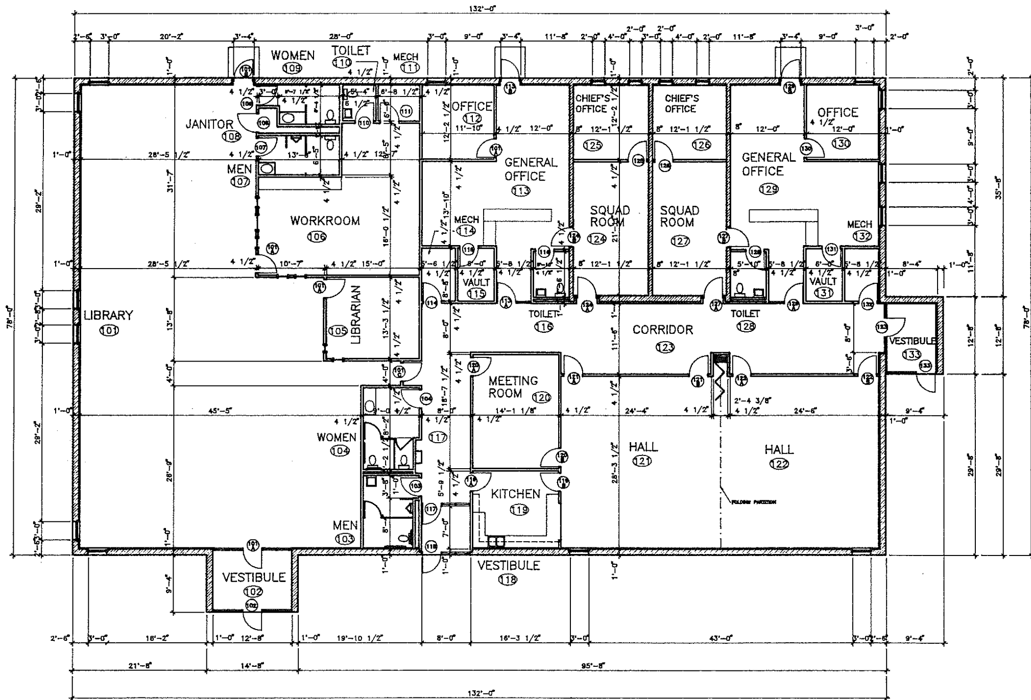
ALTERNATE FLOOR PLAN 1/8" = 1'-0"
