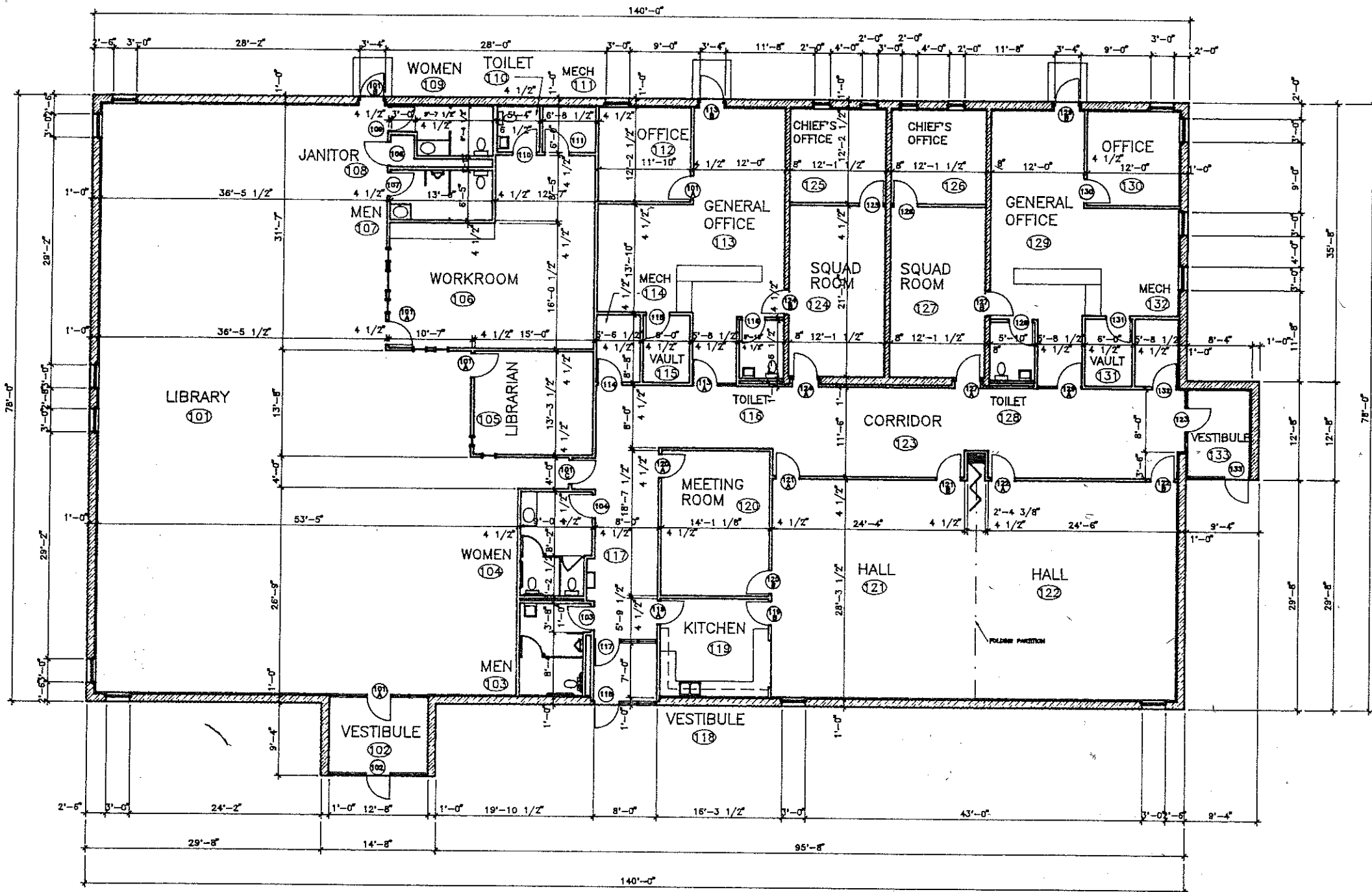
FLOOR PLAN 1/8" = 1'-0"
