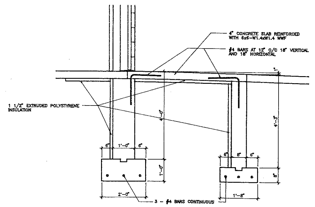
SECTION 3 3/8" = 1'-0" (S10)
