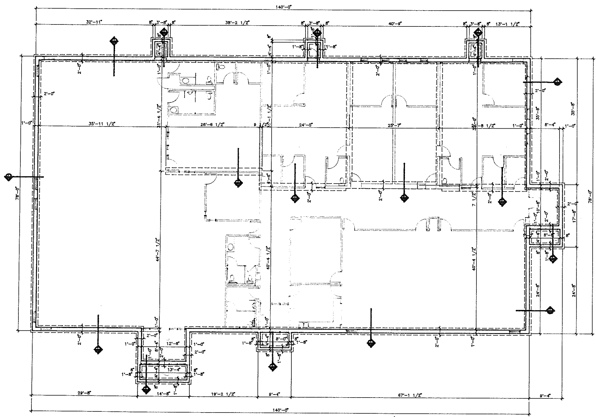
FOUNDATION PLAN 1/8" = 1'-0"
