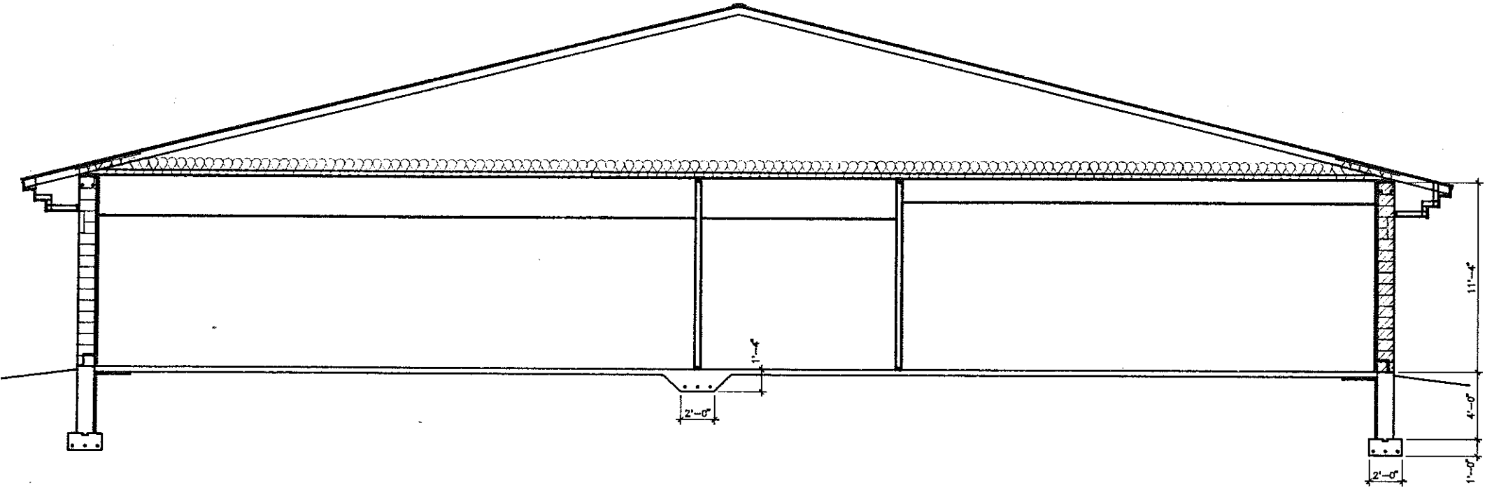
SECTION 4 1/4" = 1'-0" A202
