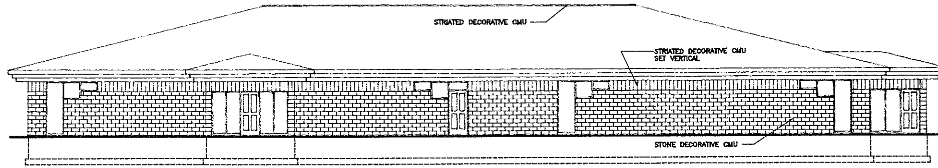
SOUTH ELEVATION 1/8" = 1'-0"
