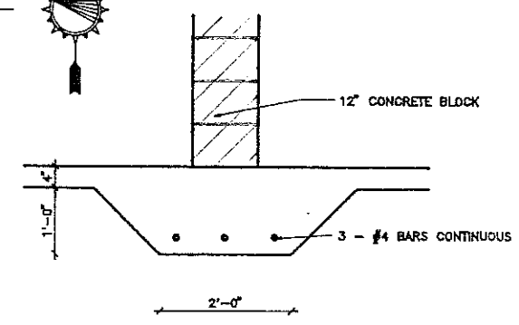
SECTION 1 3/8" = 1'-0" (S10)
