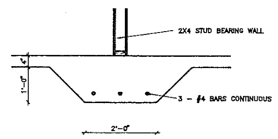
SECTION 2 3/8" = 1'-0" (S10)
