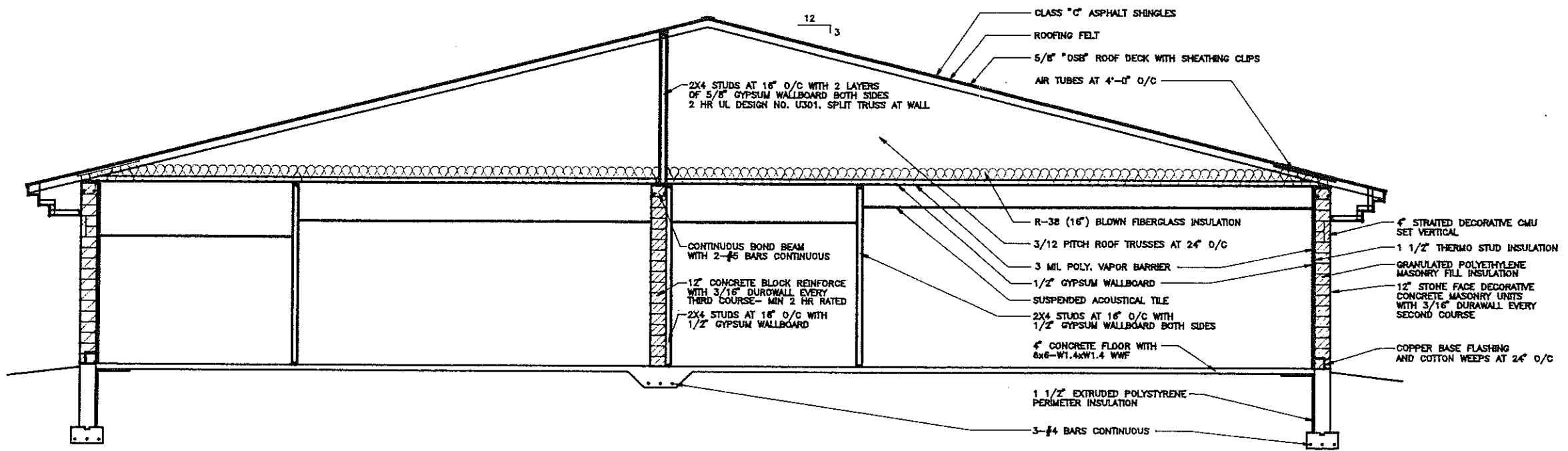
SECTION 2 1/4" = 1'-0" A202
