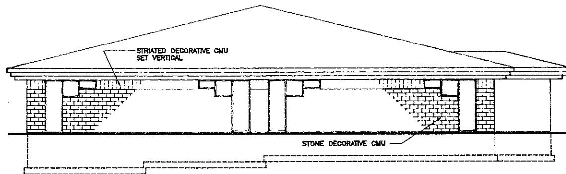
WEST ELEVATION 1/8" = 1'-0"
