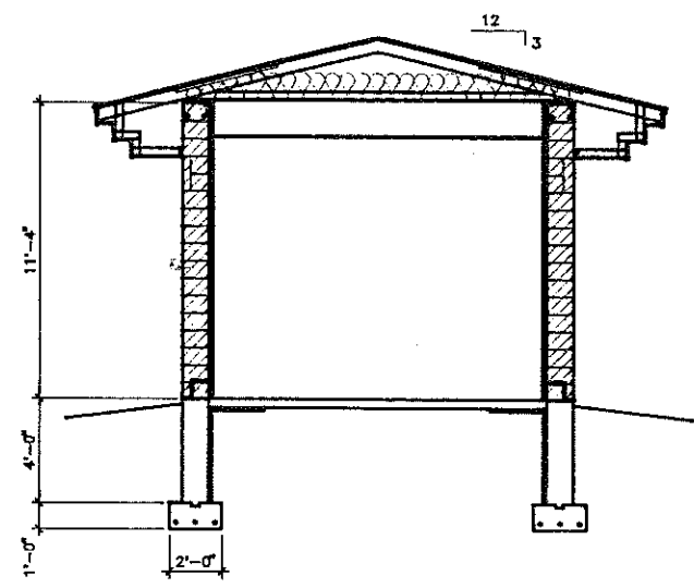
SECTION 1 1/4" = 1'-0" A202
